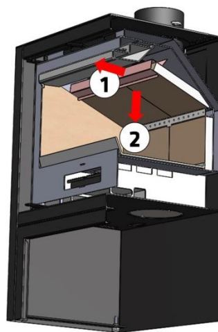
Figure No.1 - Dismantling the deflector Platinum 600
