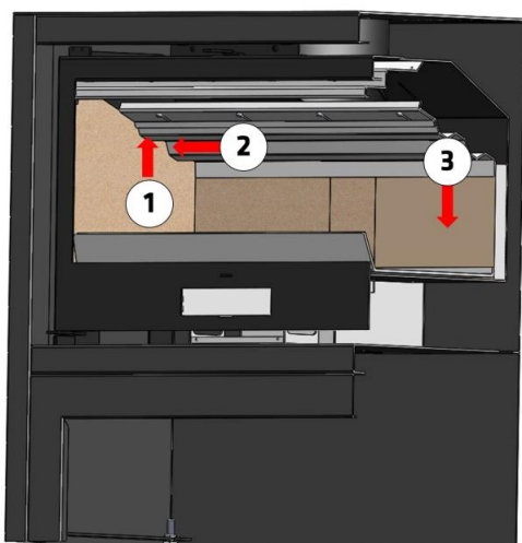
Figure No.19 - Dismantling the deflector Platinum 800
