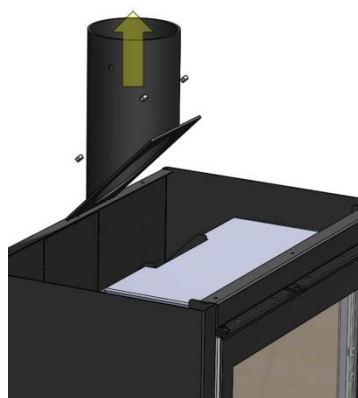
Figure No.6 - Release the smoke outlet and pull up.
