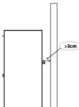
Figure No.12 - Separation between the appliance and the rear wall
