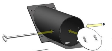
Figure No.8 - Assemble the flapper valve
