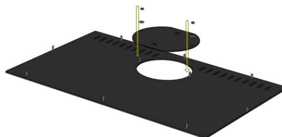
Figure No.10 - Assemble the top of the worktop with nuts and washers.
