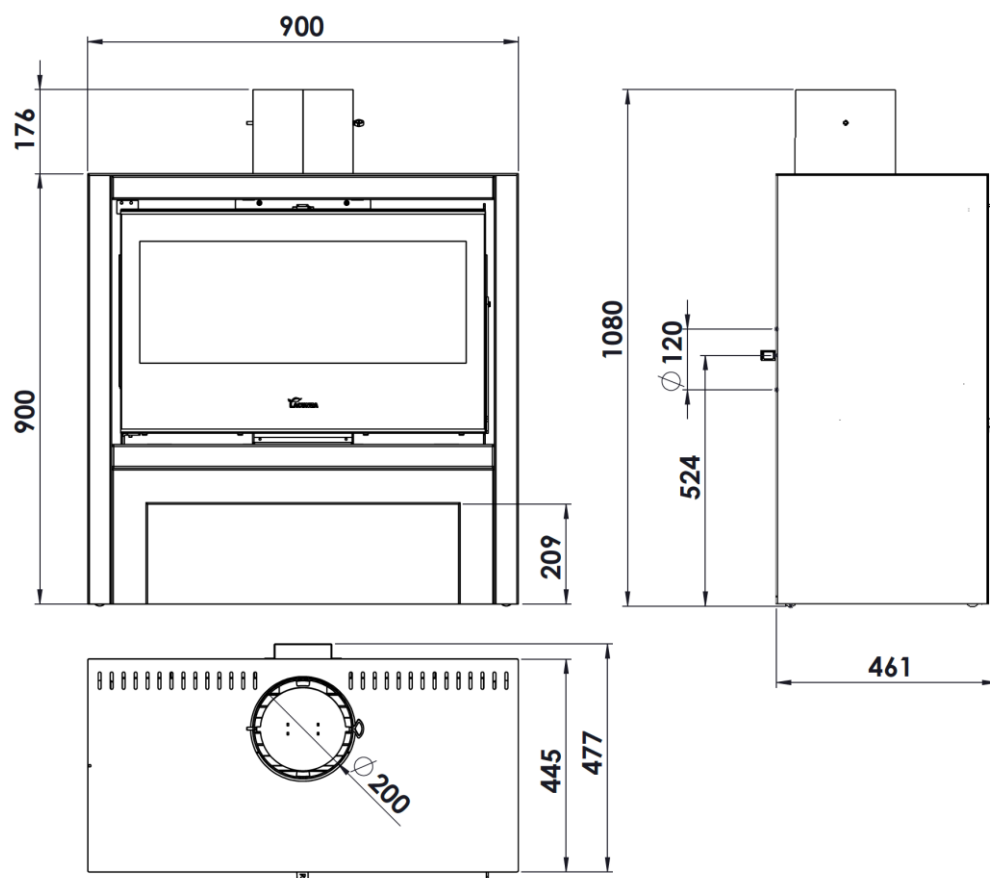
Figure No.2 - Dimensions of the PLATINUM 800 appliance in mm
