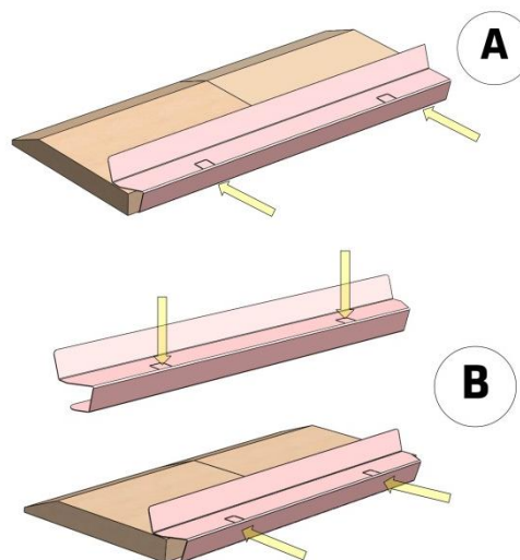
Figure No.1 - Different lower deflector positions Platinum 600
