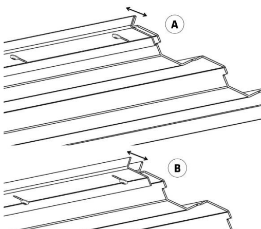
Figure No.18 - Different lower deflector positions Platinum 800
