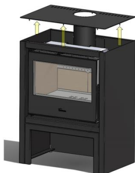
Figure No.5 - Lift countertop (no screws)
