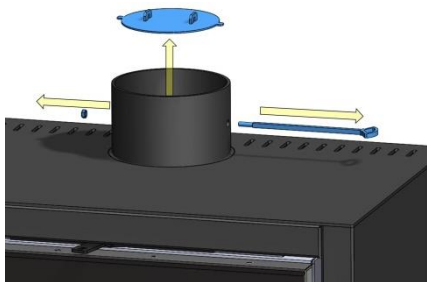
Figure No.4 - Disassemble the flapper valve
