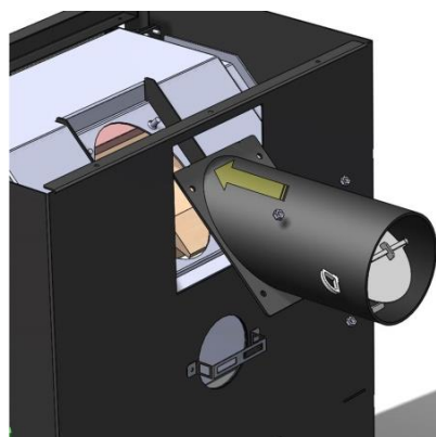
Figure No.9 - Place the smoke outlet from the back
