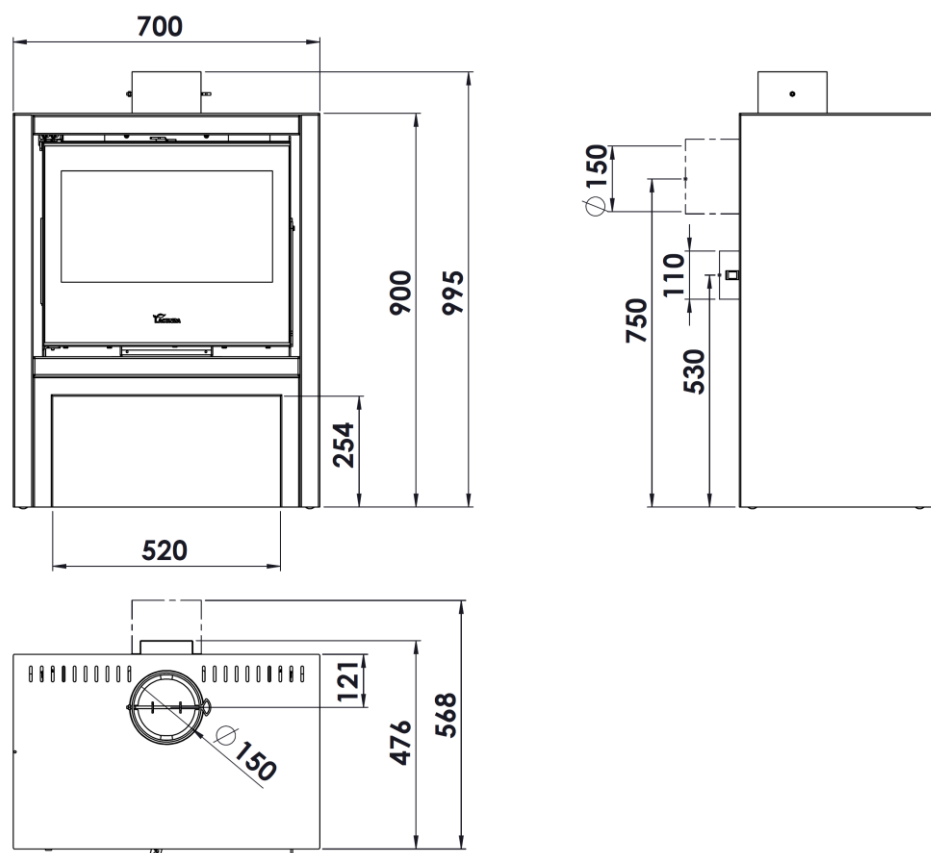
Figure No.1 - Dimensions of the PLATINUM 600 appliance in mm
