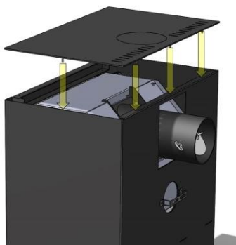
Figure No.11 - Position the countertop, by its own weight without screws.
