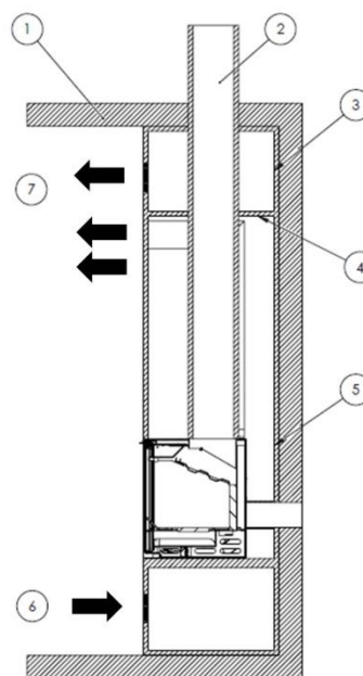
Figure No.7 - Interior diagram of the casing
