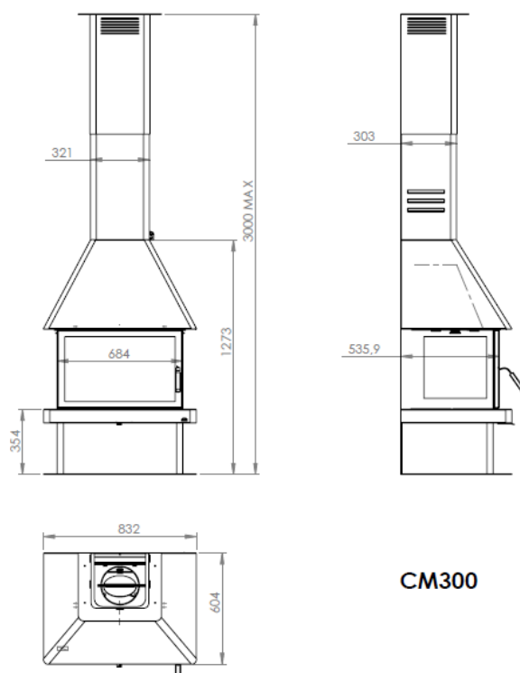
Figure No.1 - Dimensions of the CM-300 appliance in mm
