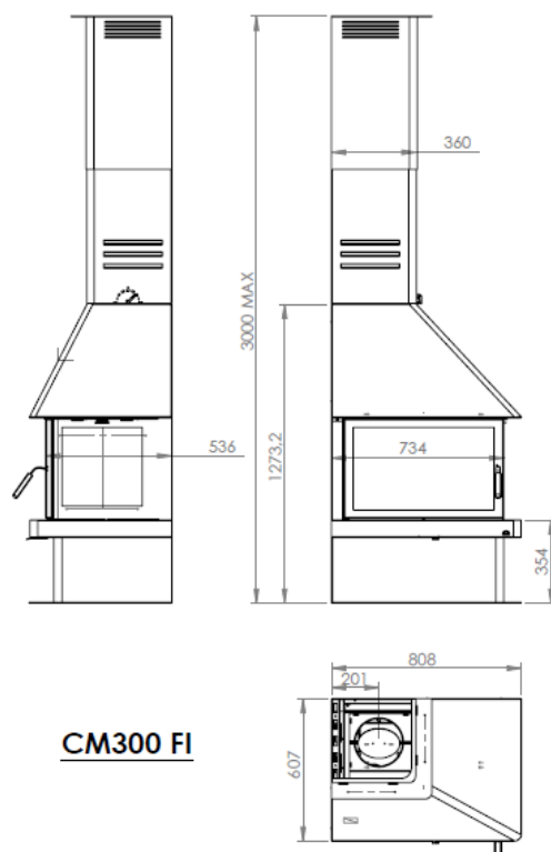
Figure No.3 - Dimensions of the CM-300 FD appliance in mm
