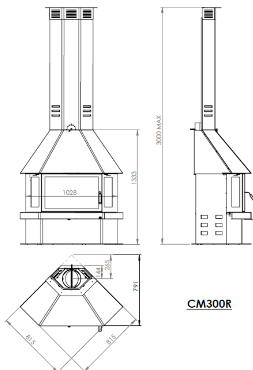
Figure No.4 - Dimensions of the CM-300 R appliance in mm
