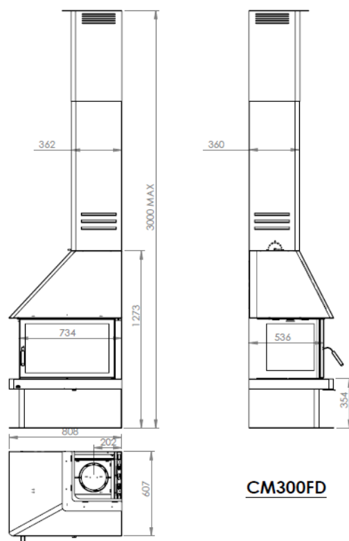
Figure No.2 - Dimensions of the CM-300 FD appliance in mm
