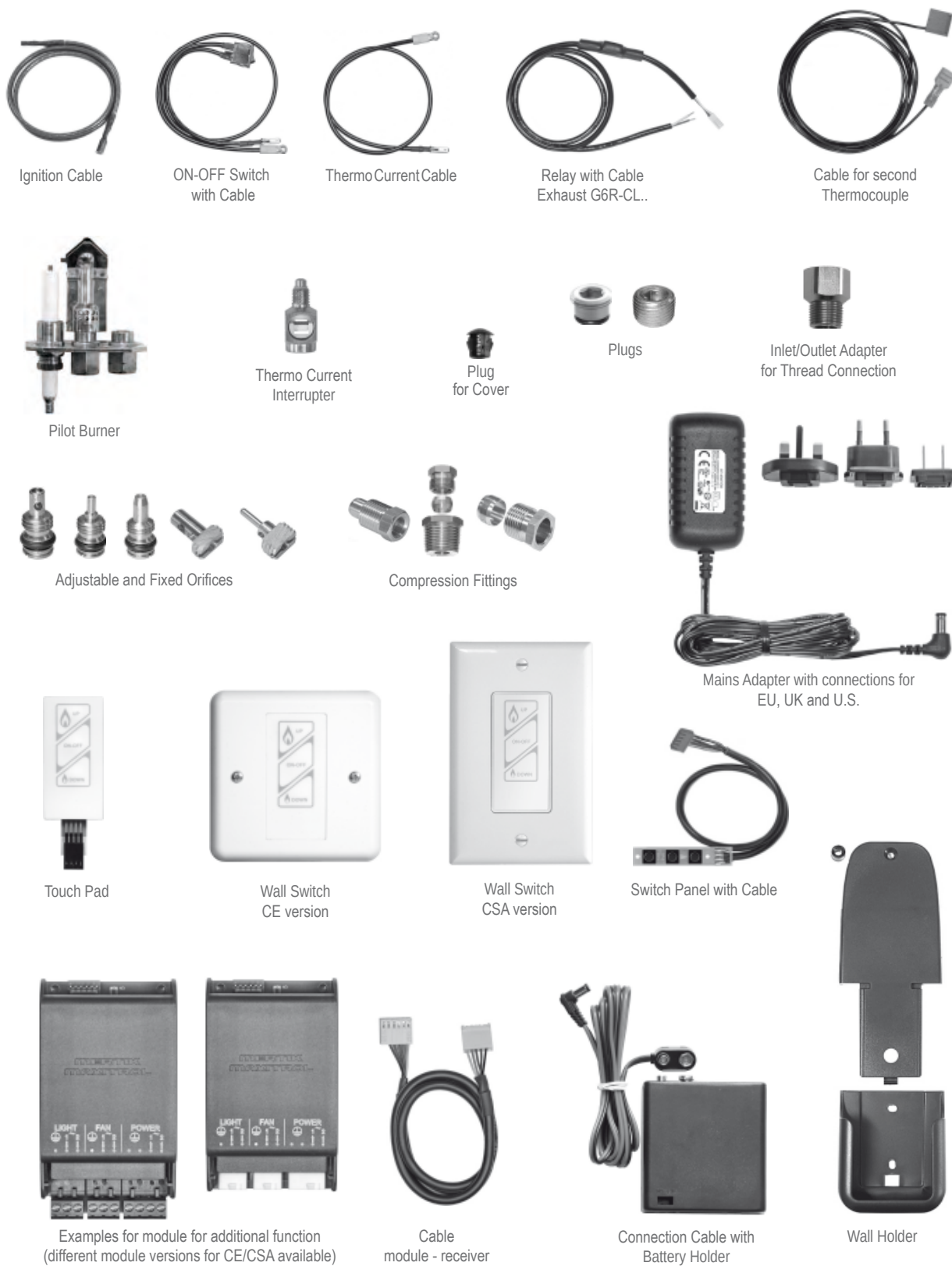
Illustration 20: GV60 Series - Accessories and Replacement Parts
