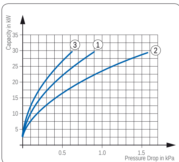
Illustration 23: Pressure Drop Diagram in kPa
