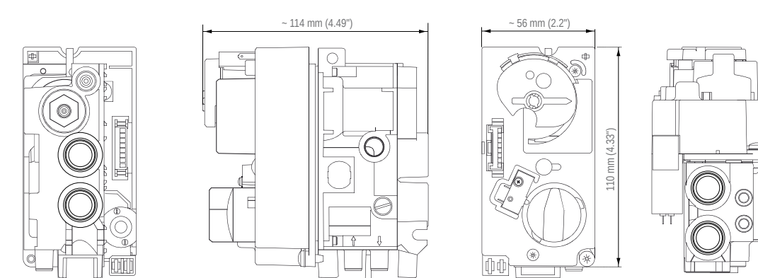
Illustration 7: GV60 Series - Dimensions and Weight
