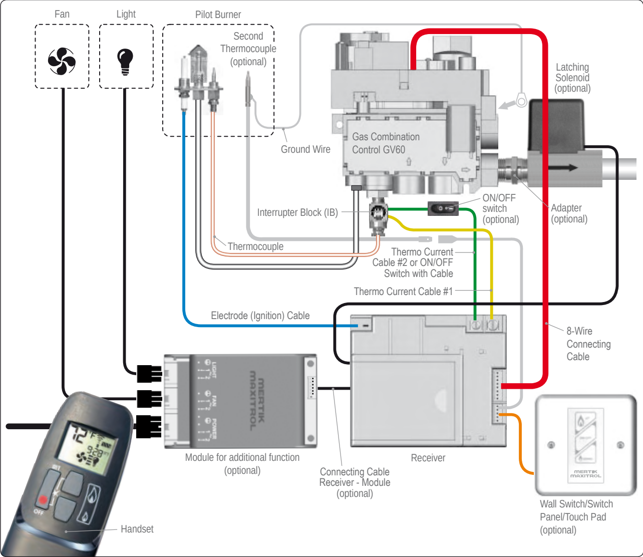
Illustration 19: GV60- Electronic Options
