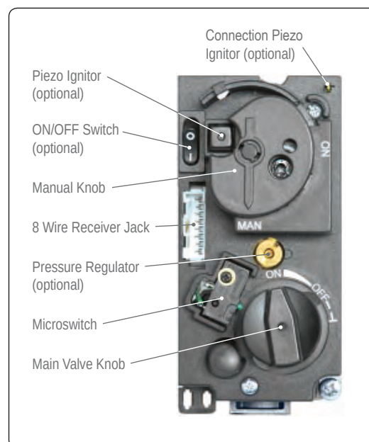
Illustration 2: GV60 - Top view
