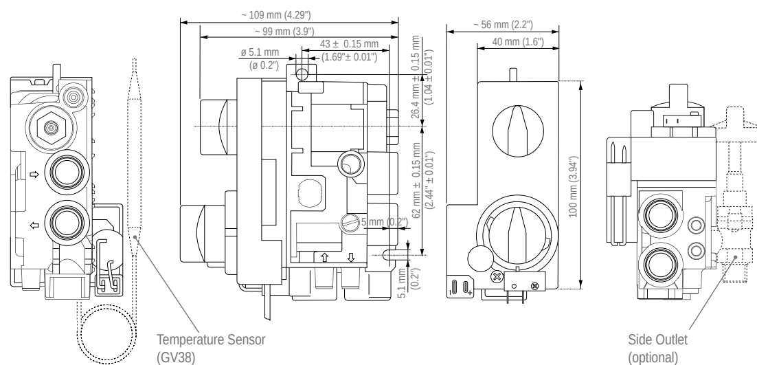
Illustration 6: GV34, 38 - Dimensions and Weight
