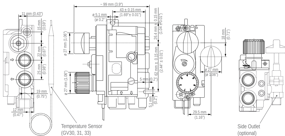
Illustration 5: GV30, 31, 32, 33, 36 - Dimensions and Weight
