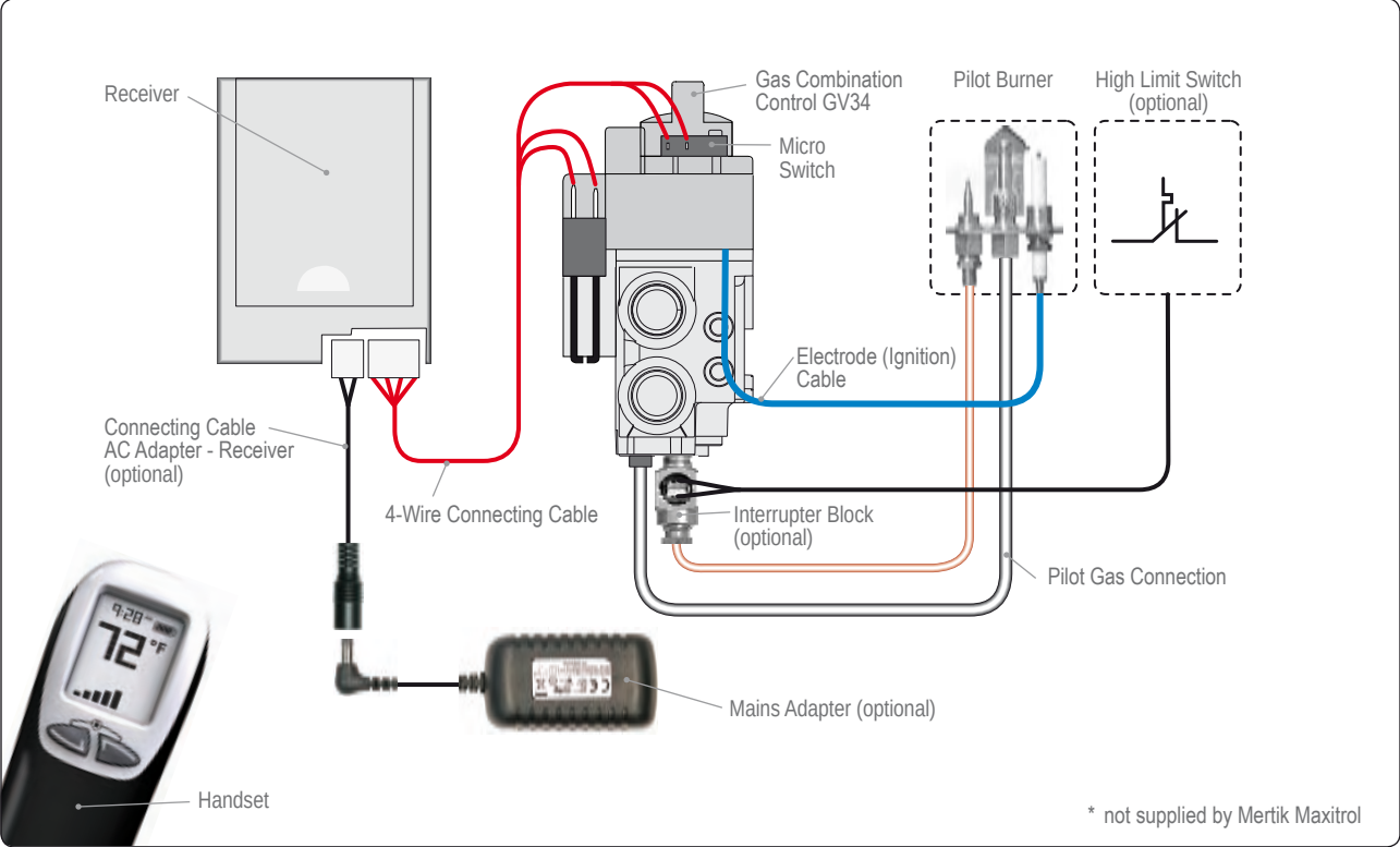
Illustration 12: GV34 - Electronic Options
